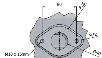
Engine Water Inlet Flange Detail Without Hose Adaptor
