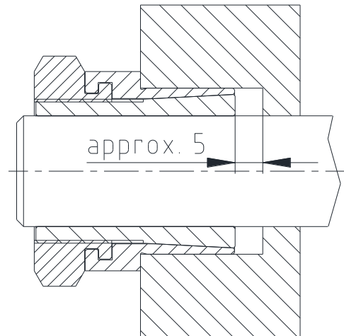
Illustration 6: Clamping set KTR 131 fully assembled
