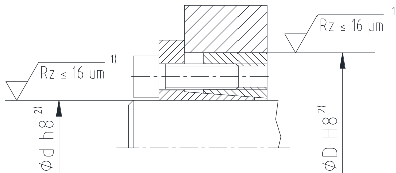
Illustration 3: Tolerances and surfaces (example: CLAMPEX® KTR 225)
